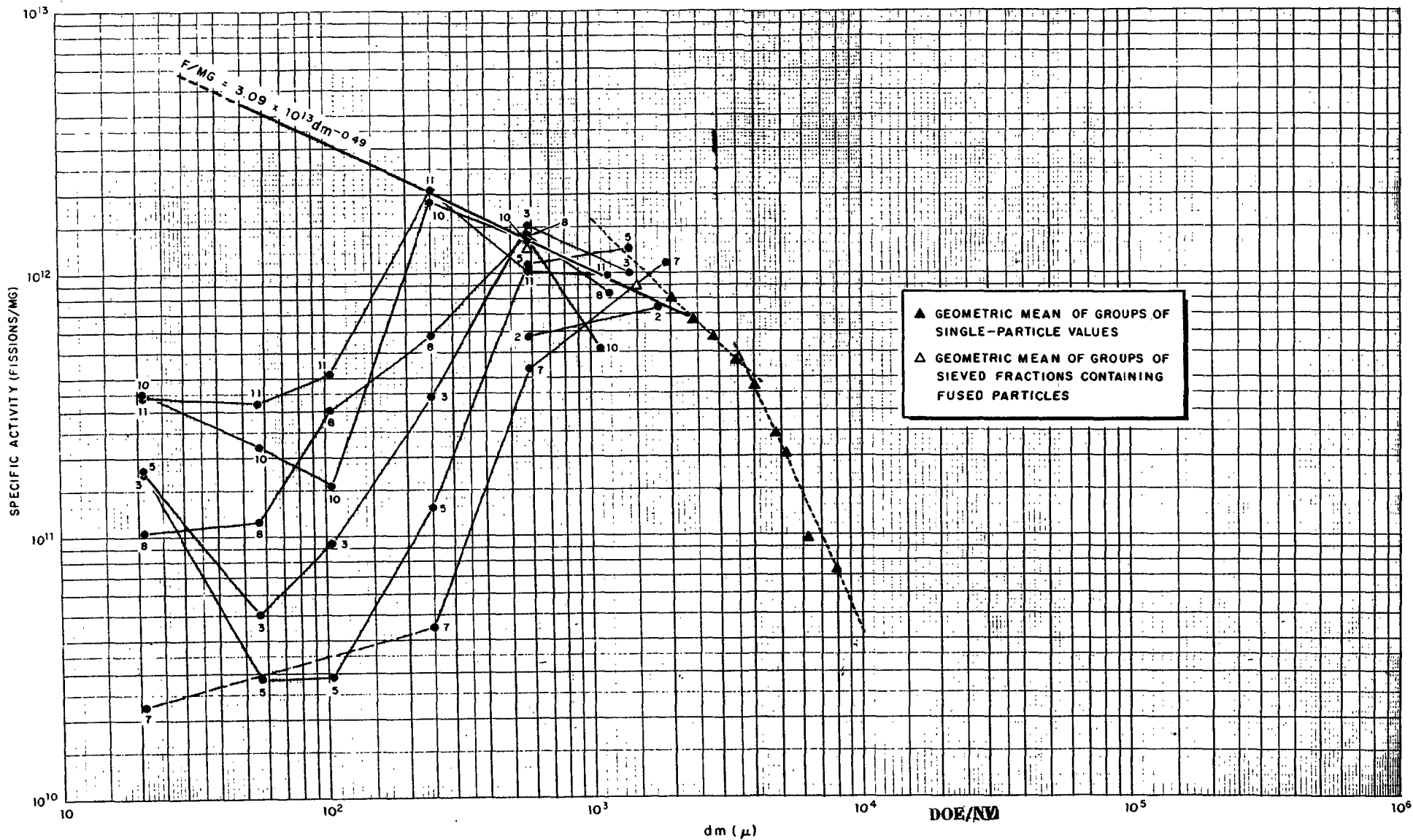
Fig. 6 Variation of Specific Activity of PLUMBBOB Shasta Fallout With Particle Size
