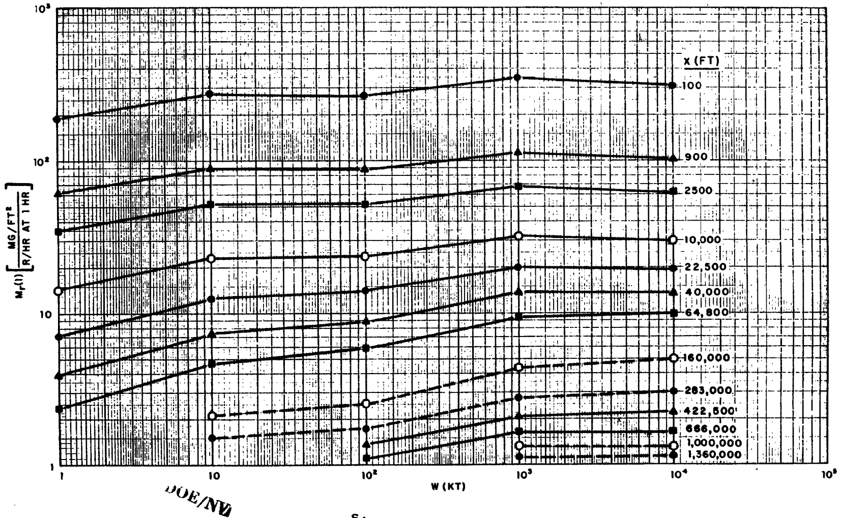
Fig. 12 Calculated Variation of M_T^S(1) as a Function of Weapon Yield for Given Values of x
