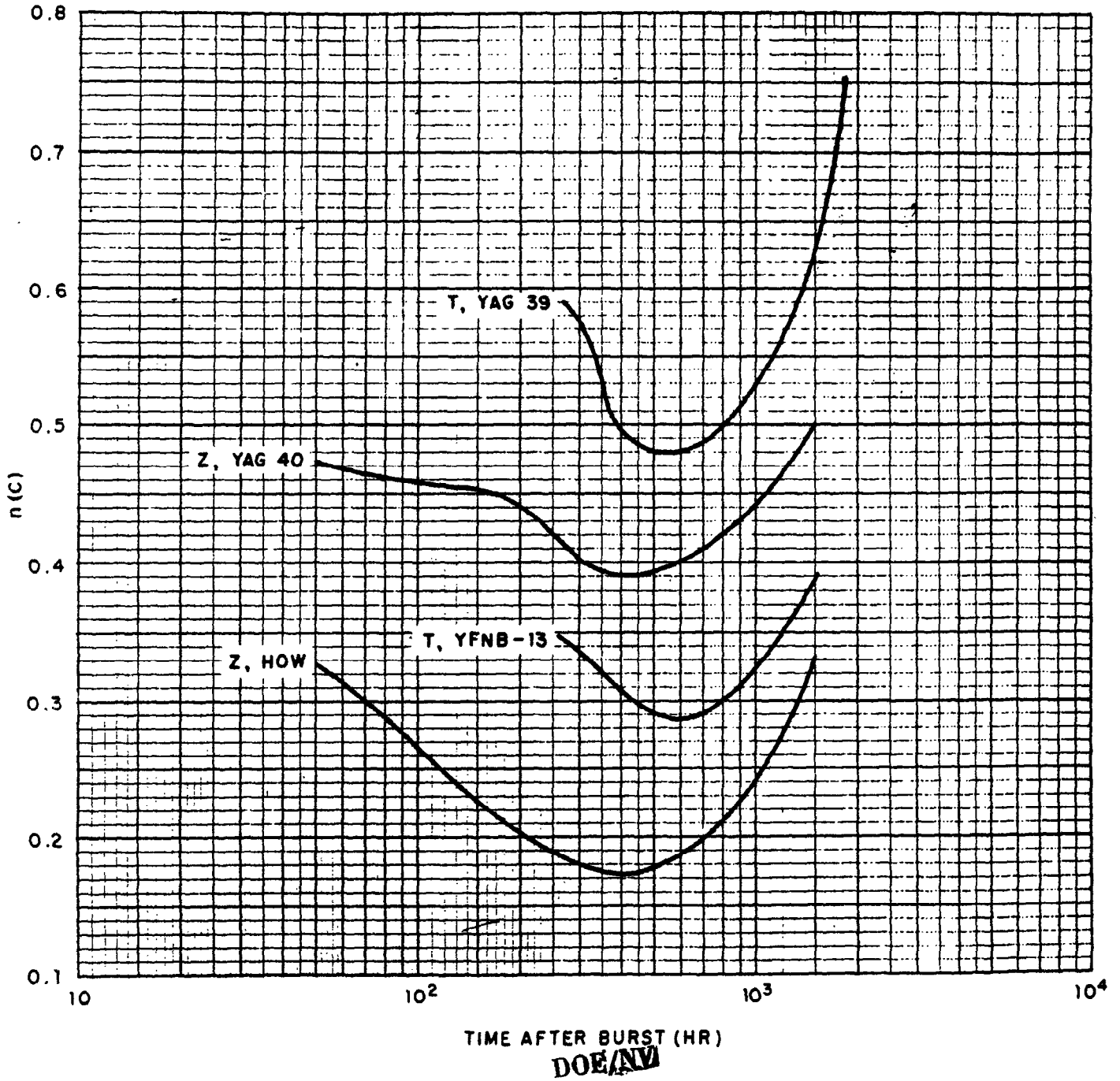
Fig. 2 Ratio of Decay Curves: Fallout Sample/Cloud Sample Based on Mo 99 Analysis
