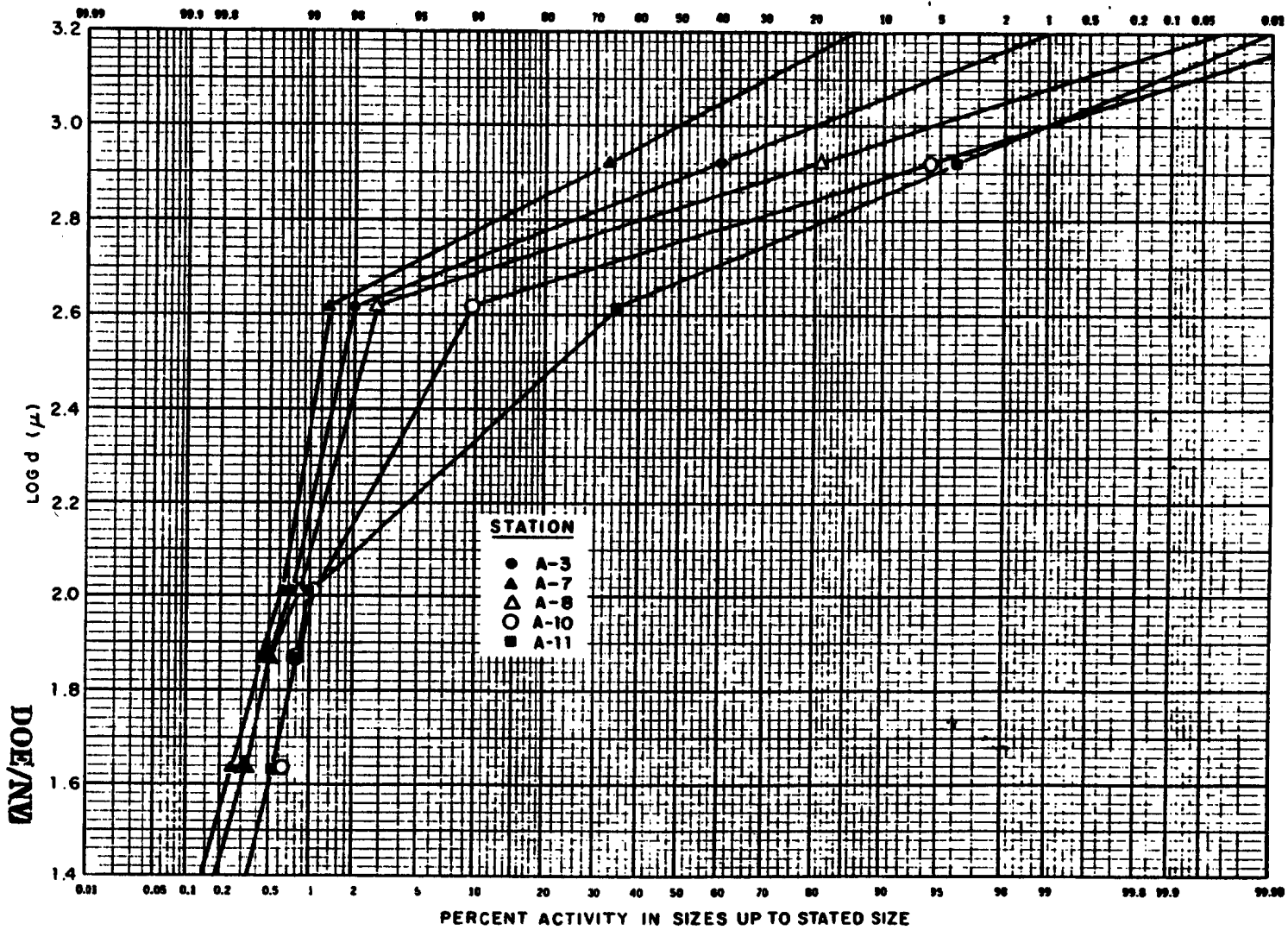
Fig. 5 Activity Size Distribution of PLUMBBOB Shasta Fallout
