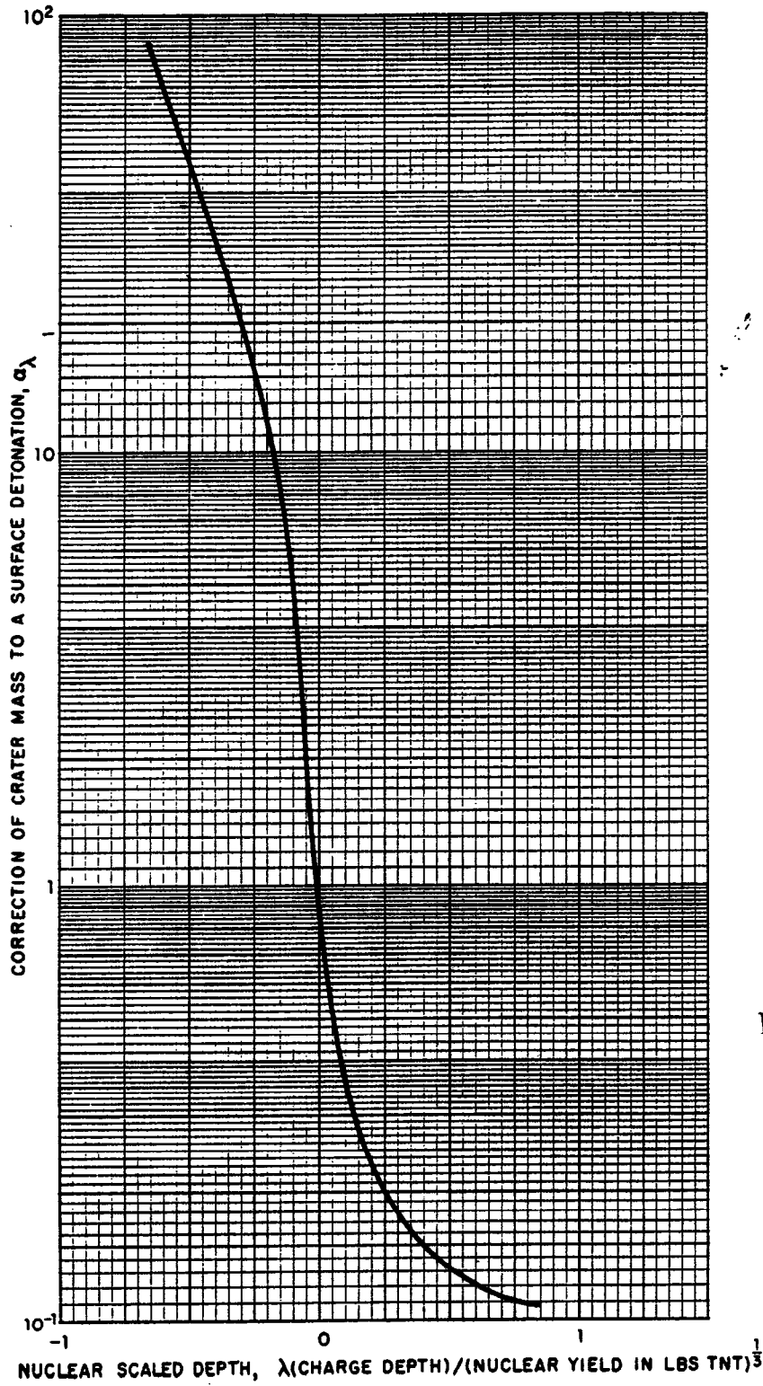
Fig. 3 Variation in \alpha_\lambda With Nuclear Scaled Depth
