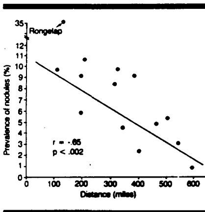
Fig 3.—Weighted linear regression. Age-adjusted prevalence of thyroid nodules weighted by inverse of population variance is plotted against distance from BRAVO test on Bikini Atoll.
