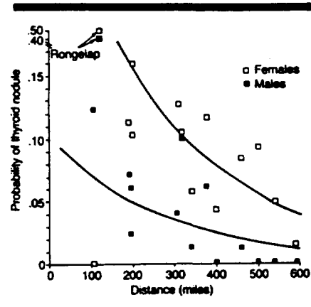
Fig 4.—Logistic regression analysis. Probability of thyroid nodule developing in an individual (from fitted logistic model) is shown for each sex, given mean age, as function of distance from Bikini Atoll. Actual prevalence data are also plotted. Females, top curve, and males, bottom curve.
