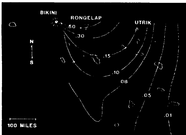
Fig 5.—Probability contours. Graph shows fitted probability contours for thyroid nodules for females, computed from complete logistic model. Distance was calculated for each contour of fixed probability, given mean age of females, for values of \theta from 0° to 80°.
