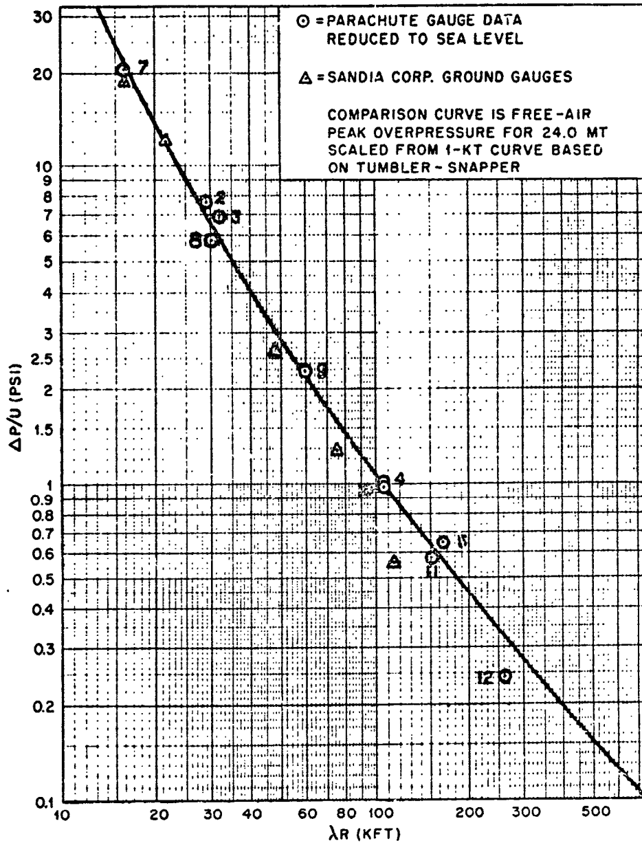
Fig. 3.7—Peak overpressure vs slant range reduced to homogeneous atmosphere at sea-level ambient pressure (Fuchs scaling), Mike suot.
