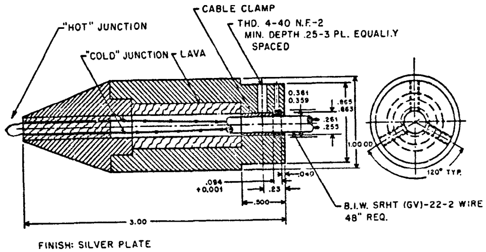
Fig. 2.1—Thermocouple housing.
