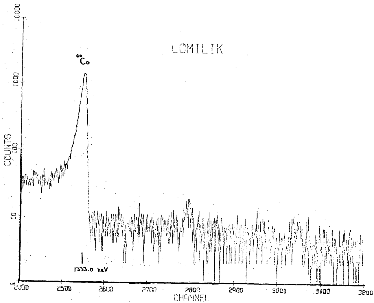
Figure 11d. Ge(Li) spectrum of soil sample taken from Lomilik Island, Aomen-Iroi Complex.
