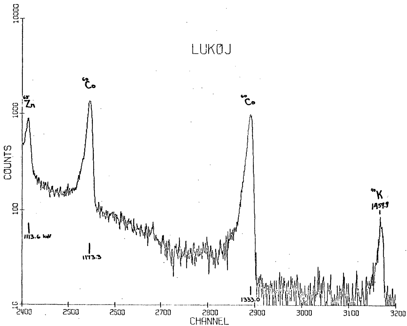
Figure 10d. Ge(Li) spectrum of soil sample taken from LukøJ Island.
