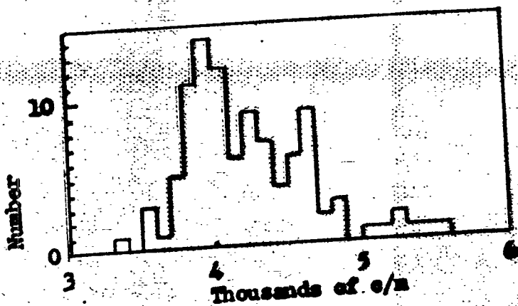
Figure 2. Histograms showing frequency distributions of counts of radioactivity of Engebi beach sand. Upper, counts for 100 small (6 mg) samples. Middle, logarithms of logarithms of the same counts. Lower, counts for 100 large (3000 mg) samples.
