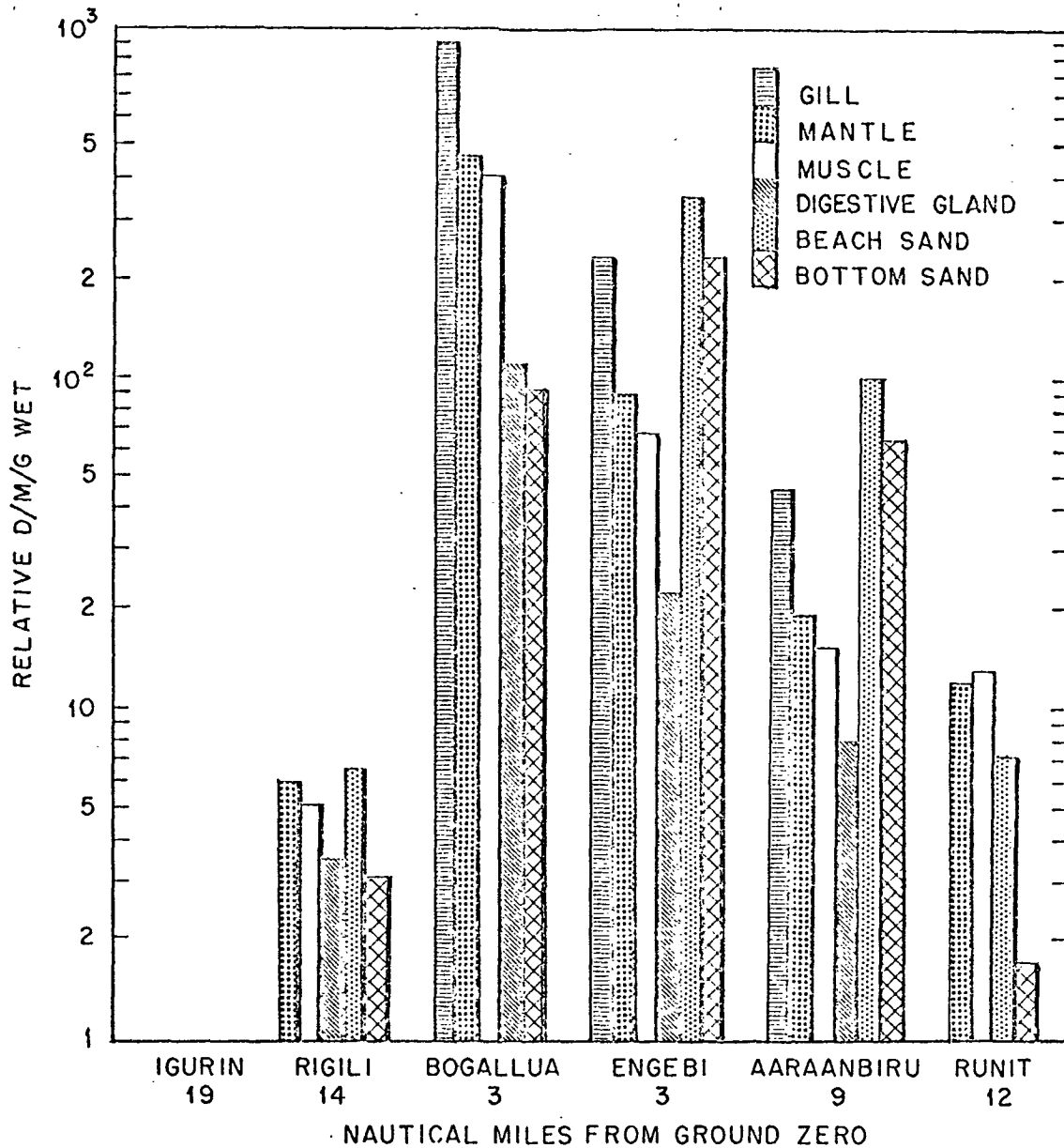
Figure 5. Relative radioactivity of soil or beach sand, bottom sand taken from sea cucumber guts and giant clam gill, mantle, muscle and digestive gland. The relative activity of each type of sample at Igurin is taken as 1 .
