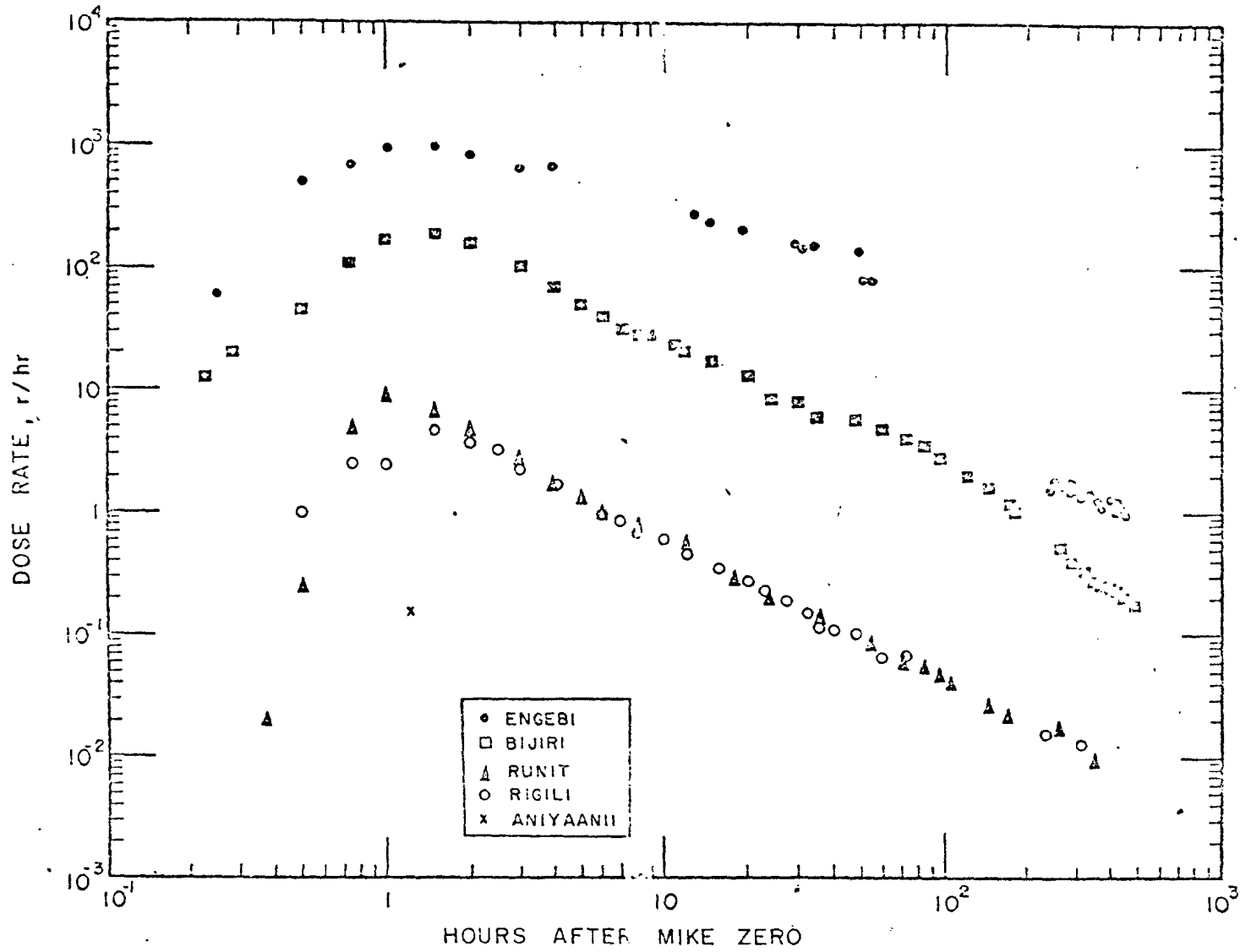
Fig. 6 - Mike fall-out intensity versus time.
