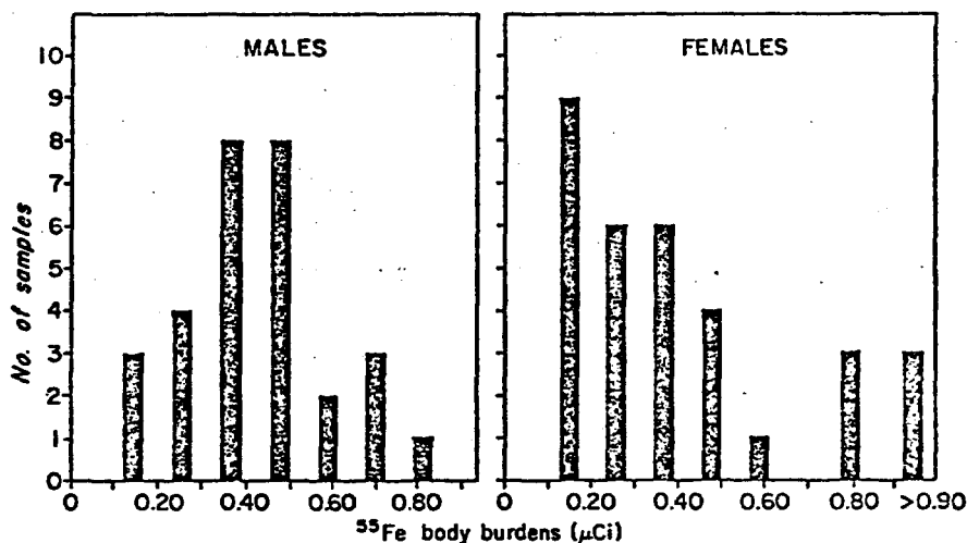
FIG. 1. Frequency distribution of ^{55}\text{Fe} body burdens in Rongelap males and females. Body burdens have been grouped into classes. Example: 3 Rongelap males had ^{55}\text{Fe} body burdens between 0.10–0.20 \mu\text{Ci} while nine females had ^{55}\text{Fe} body burdens in the same activity interval.
