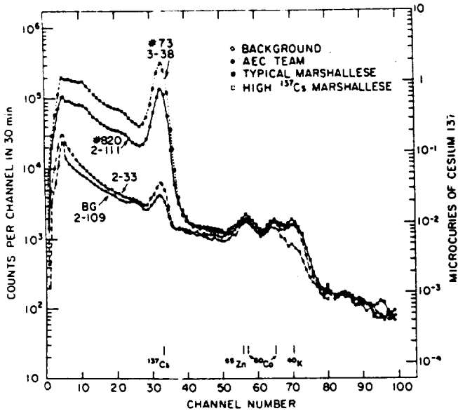
Figure 69. Unprocessed gamma-ray spectrographs obtained with an 11½-in. NaI (Tl) crystal in a shadow-shield whole-body counter. The channel width was 20 keV. Traces of 137 Cs and 60 Co are apparent in the background spectrum. The right-hand scale was obtained by calibration with a "standard man" phantom and requires correction for other body sizes; it is adjusted for the 137 Cs peak.
