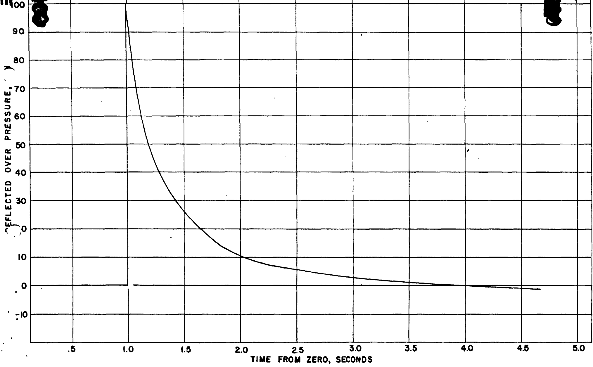
FIGURE 4 PRESSURE VS TIME RANGE 6500' 5MT SURFACE BUR IDEAL SURFACE
