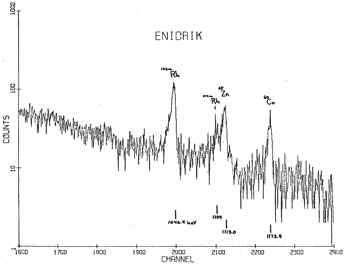
Figure 9c. Ge(Li) spectrum of soil sample taken from Enidrik Island.
