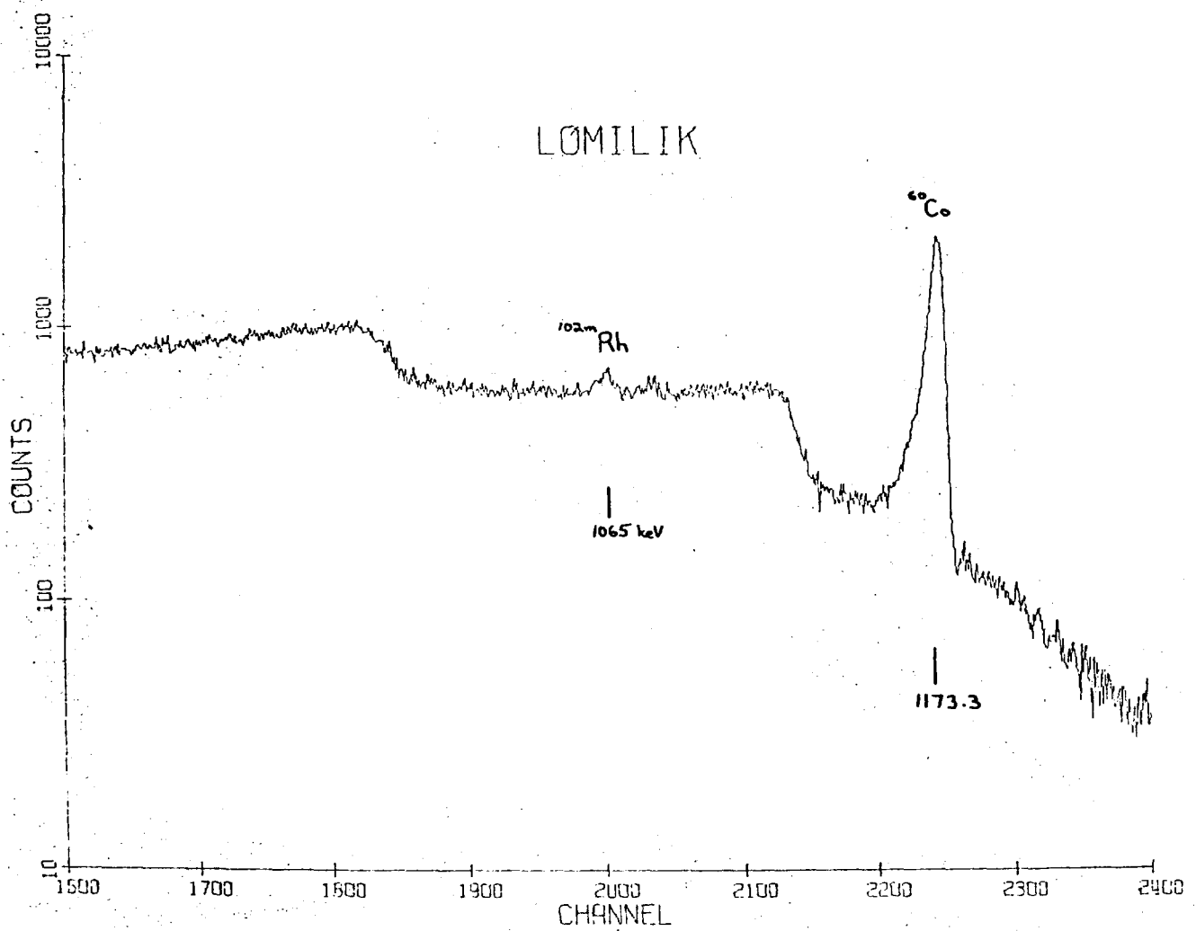
Figure 11c. Ge(Li) spectrum of soil sample taken from Lomilik Island, Aomen-Iroi Complex.
