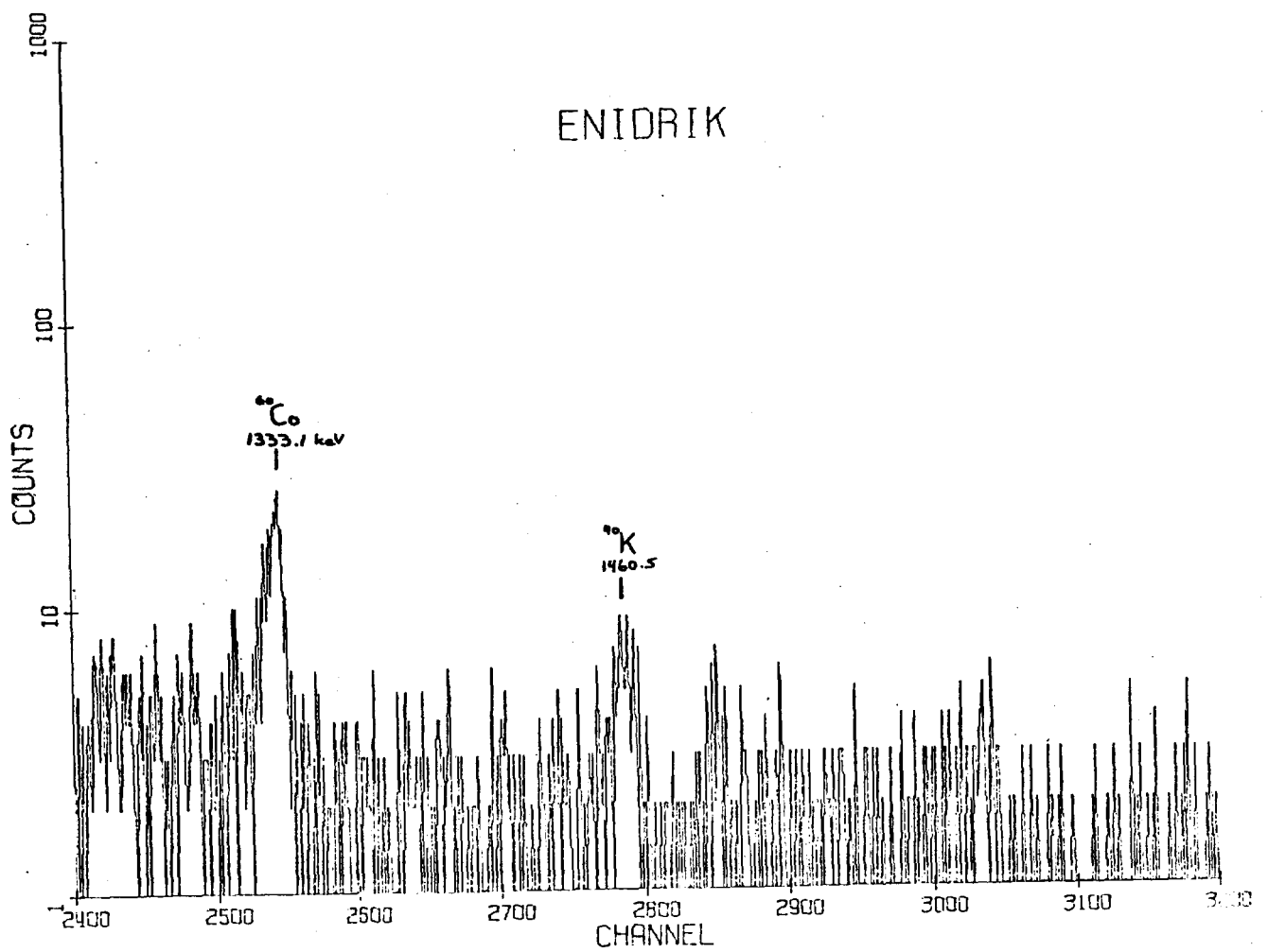
Figure 9d. Ge(Li) spectrum of soil sample taken from Enidrik Island.
