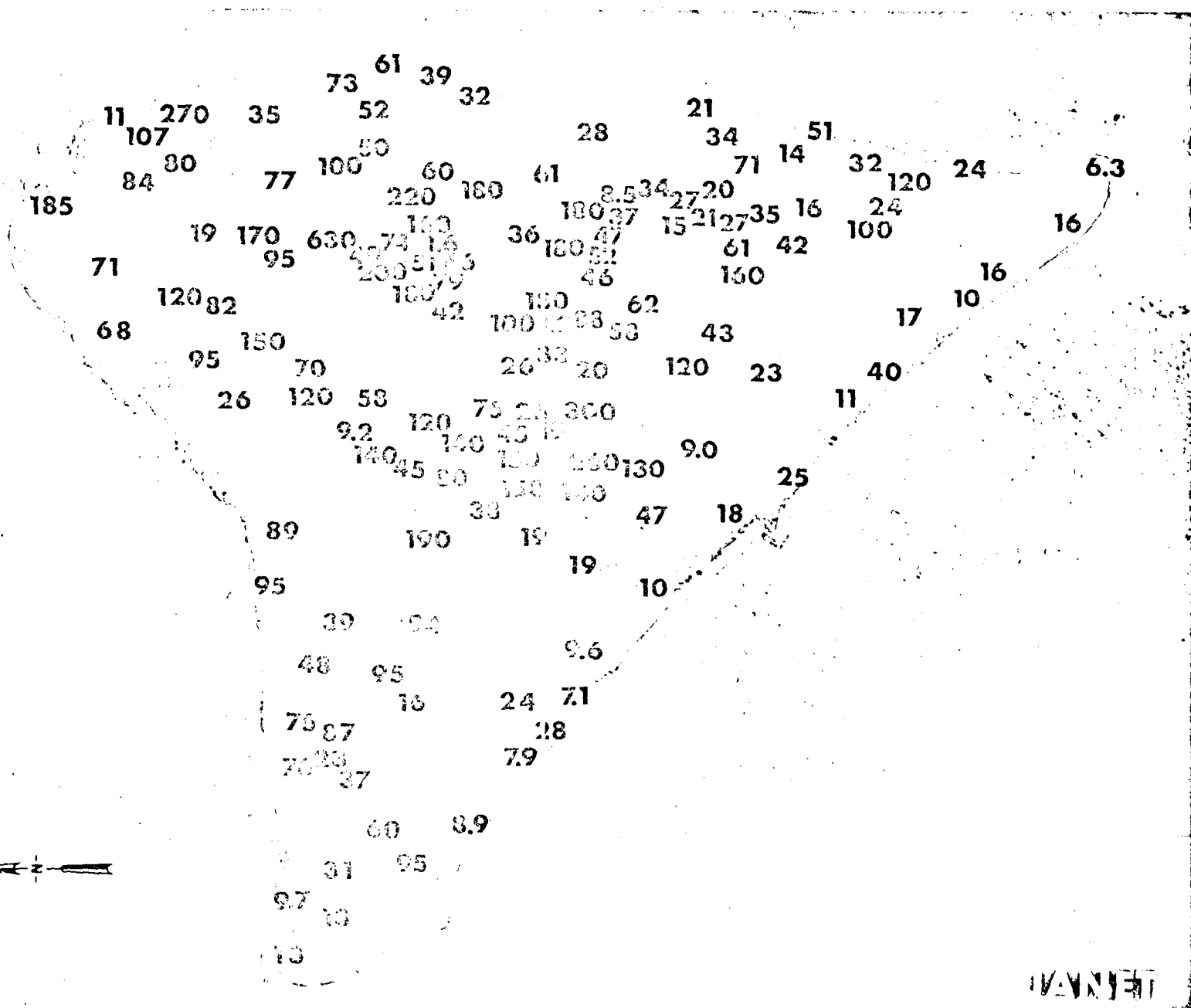
The average 90 Sr activities (pCi/gm) in soil samples collected to a depth of 15 cm.
