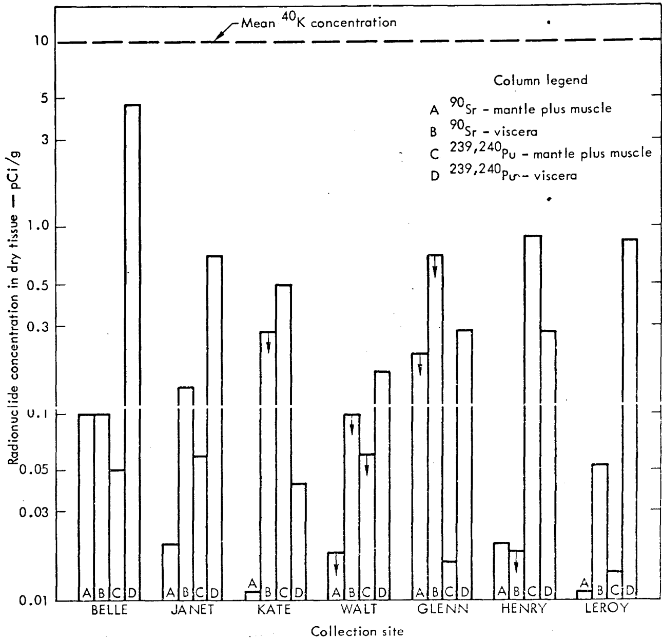
Fig. 165. Average 90 Sr and 239,240 Pu concentration in the viscera, mantle, and muscle of Tridacna clams collected at Enewetak Atoll, October to December, 1972. The 40 K value is the mean for all Tridacna samples.
