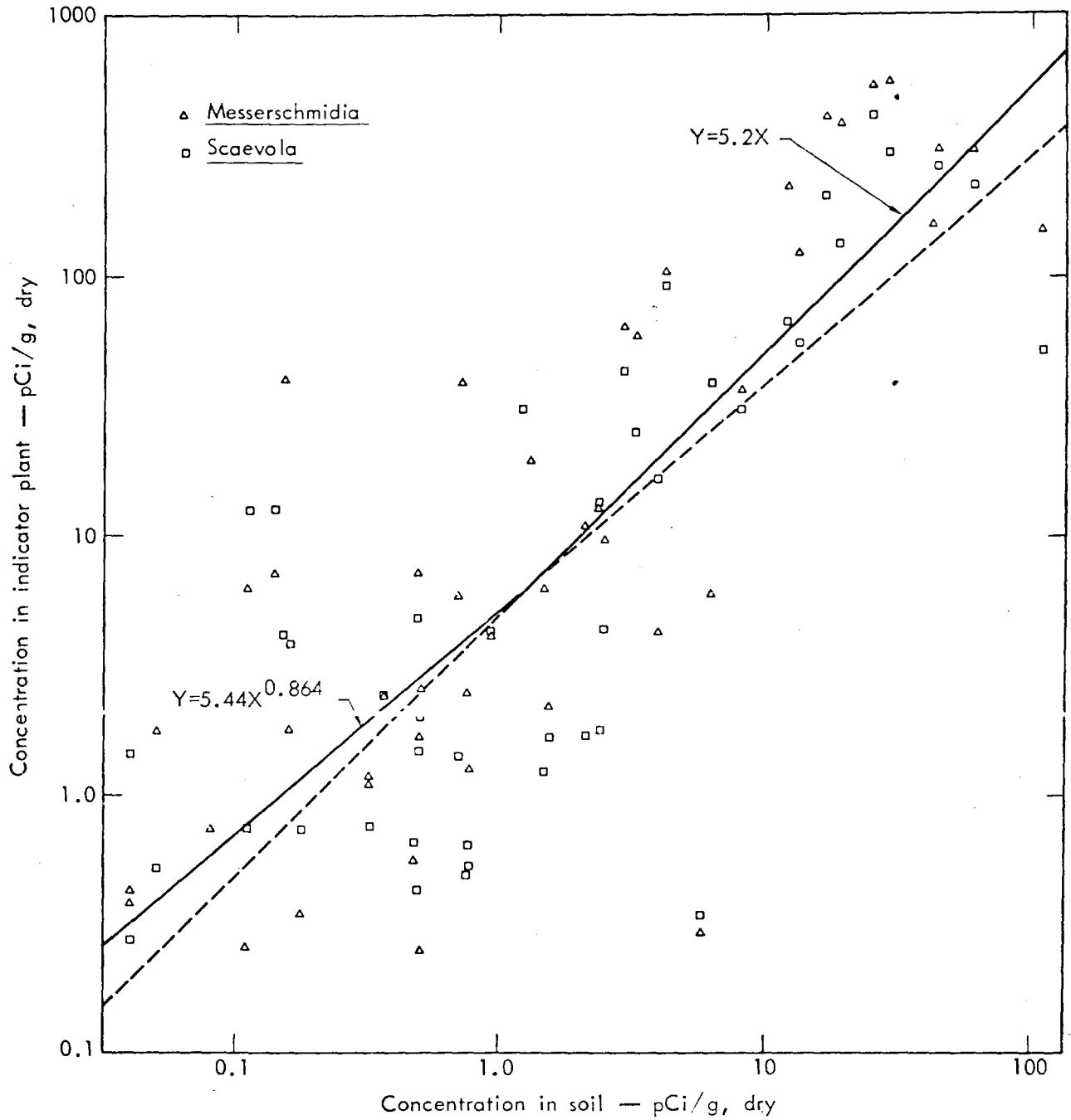
Fig. 169. Statistical correlation between 137 Cs in Messerschmidia and Scaevola and 137 Cs in soil.
