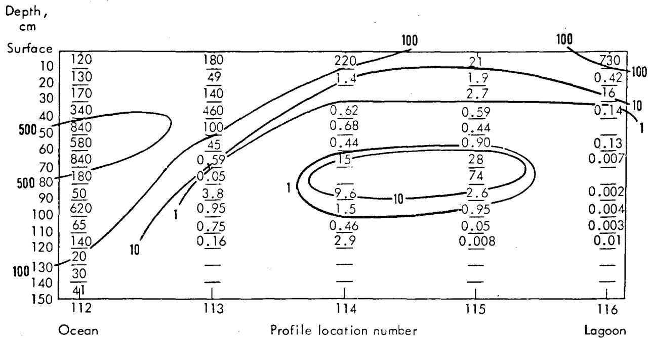
Fig. 155. Plutonium profile data, Locations 112-116, YVONNE.
