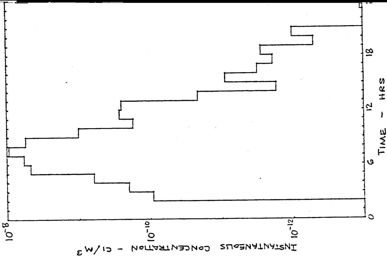
Figures 3d. Same as Fig. 3a, exc
