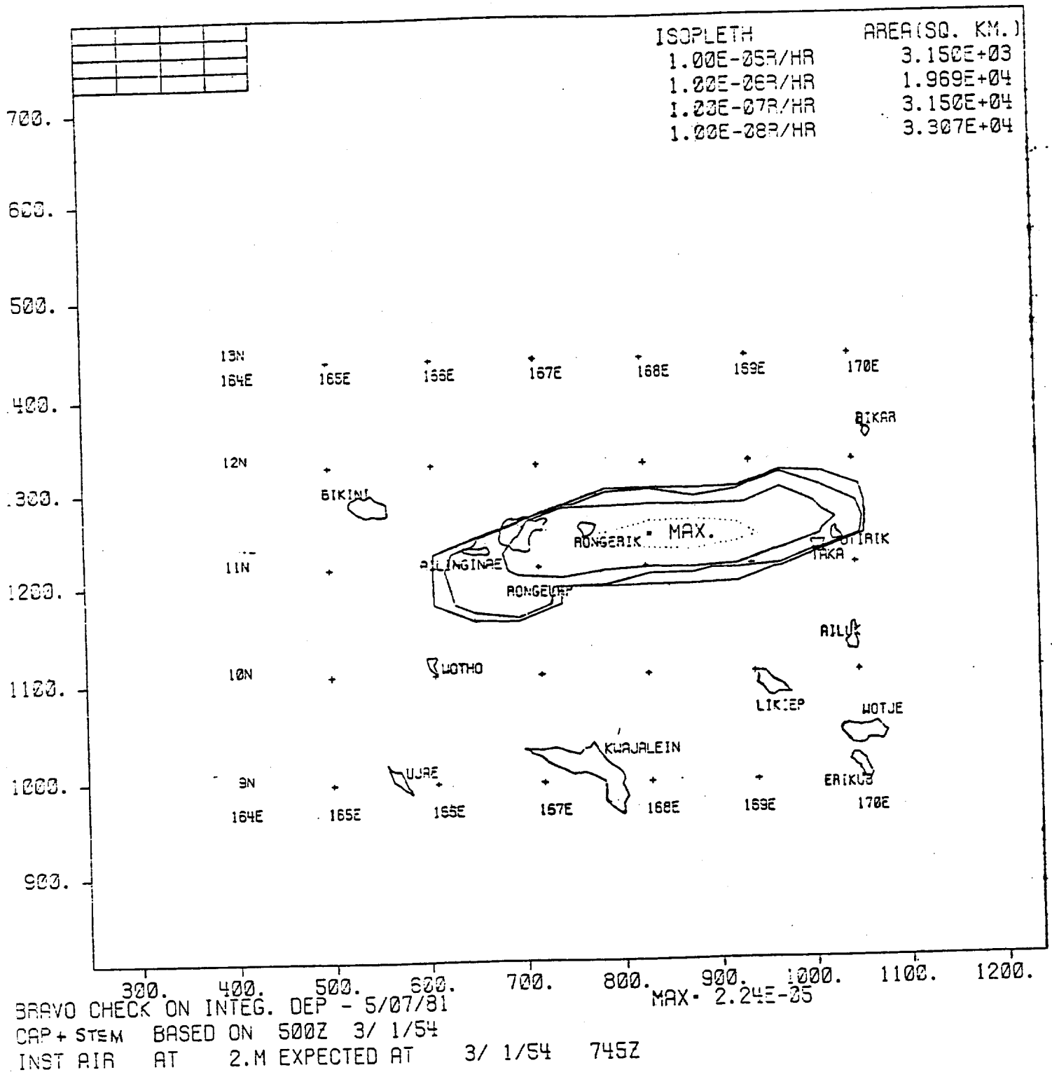
Figure 2e. Same as Fig. 2a, except time is H+13 hours.
