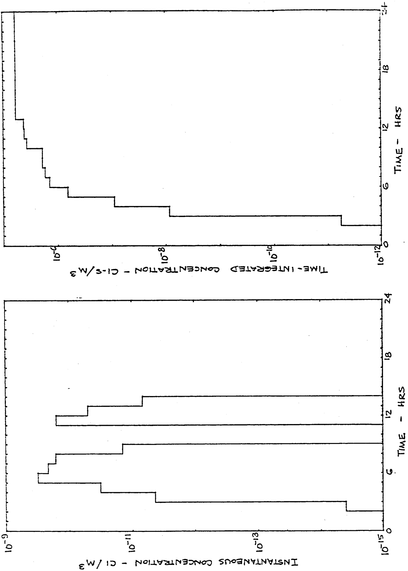
Figure 5d. Same as Fig. 5a, except nuclide is cesium-137.
