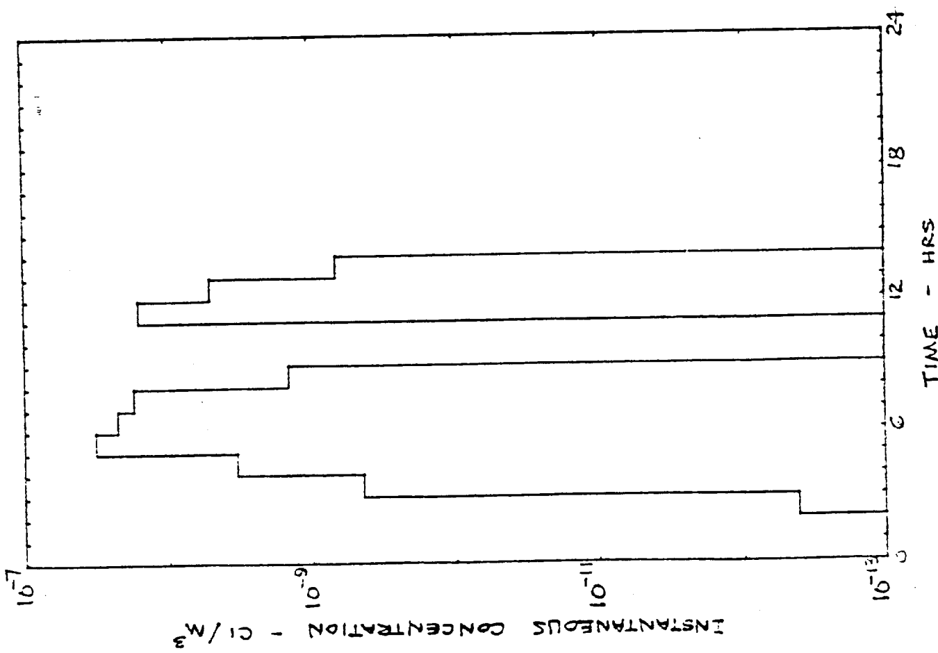
Figure 5b. Same as Fig. 5a, except nuclide is iodine-131.
